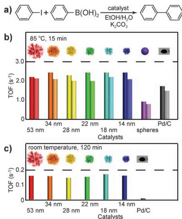
Figure 4. TOF values of the Pd-based catalysts for the coupling reaction between iodobenzene and phenylboronic acid. a) Reaction equation. b) TOF values at 85 °C for 15 min. For each catalyst, the left column shows the TOF value in the first run, and the right one indicates the TOF value in the second run. c) TOF values at room temperature for 120 min.
